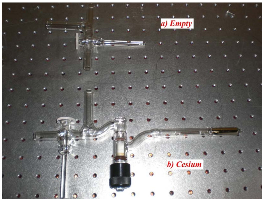
Figure 3.8. a) The basic mount used at the vacuum side of the setup. b) The cesium mount was more elaborate, taking the basic mount and adding a valve and the break-seal ampoule.
