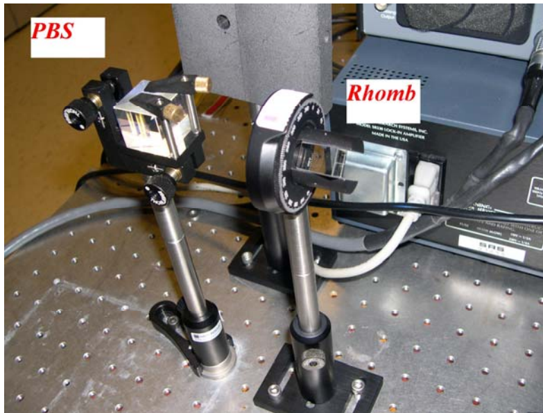
Figure 3.4. A polarizing beam splitter and a rhomb, acting as a quarter waveplate, protect the laser against damaging back reflection.
